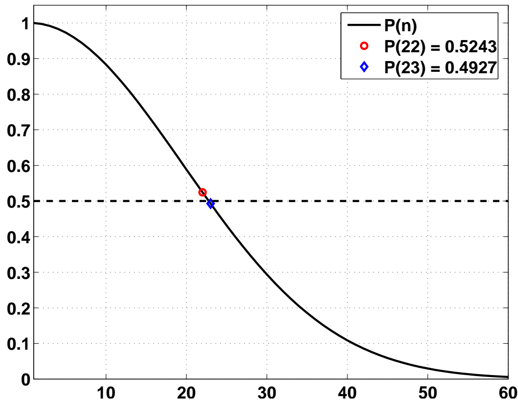
P(n) : The Probability for Different Birthdays
