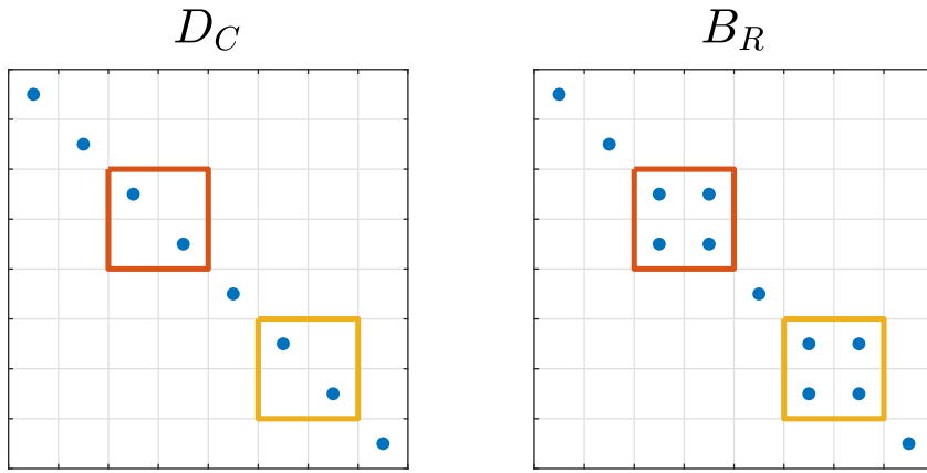
Figure: The (2 \times 2) blocks in D_{\mathbb{C}} \in \mathbb{C}^{n \times n} contain complex pairs of eigenvalues; and the corresponding blocks in B_{\mathbb{R}} \in \mathbb{R}^{n \times n} contain “rotation blocks.”
