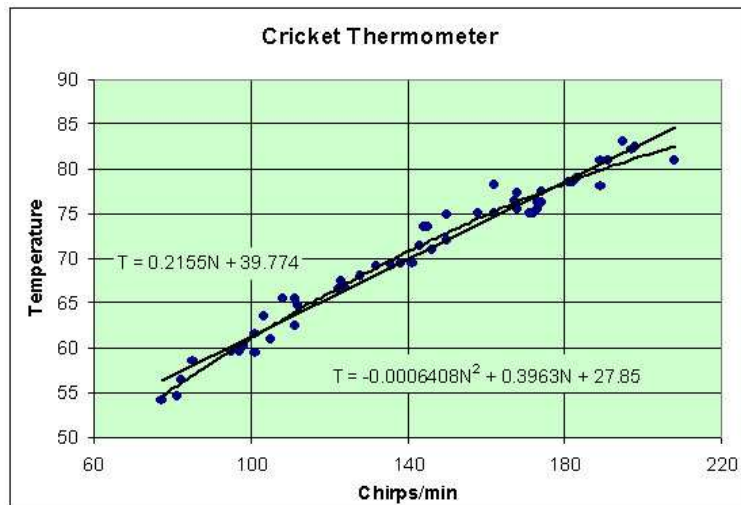
Quadratic Fit
