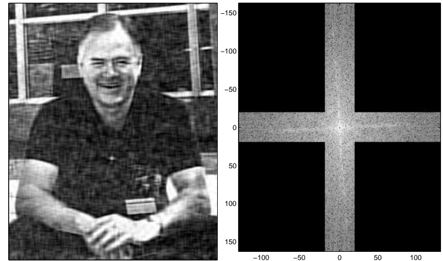
Figure: Here, we filter out \sim 75\% of the Fourier coefficients, and reconstruct the image.
