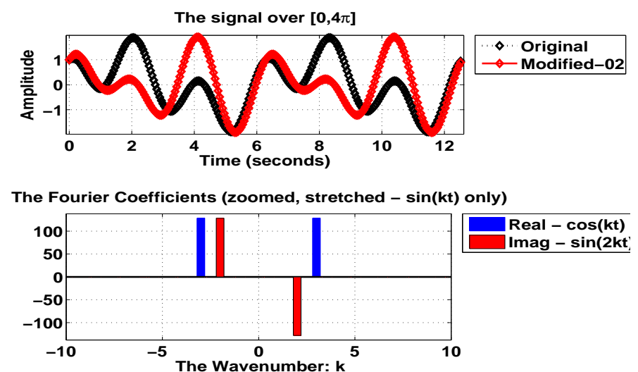
Figure: BOTTOM~ Here, we have moved the sin-coefficients from position k to position 2k . TOP~ The function f_2(t) reconstructed from the modified Fourier coefficients.
