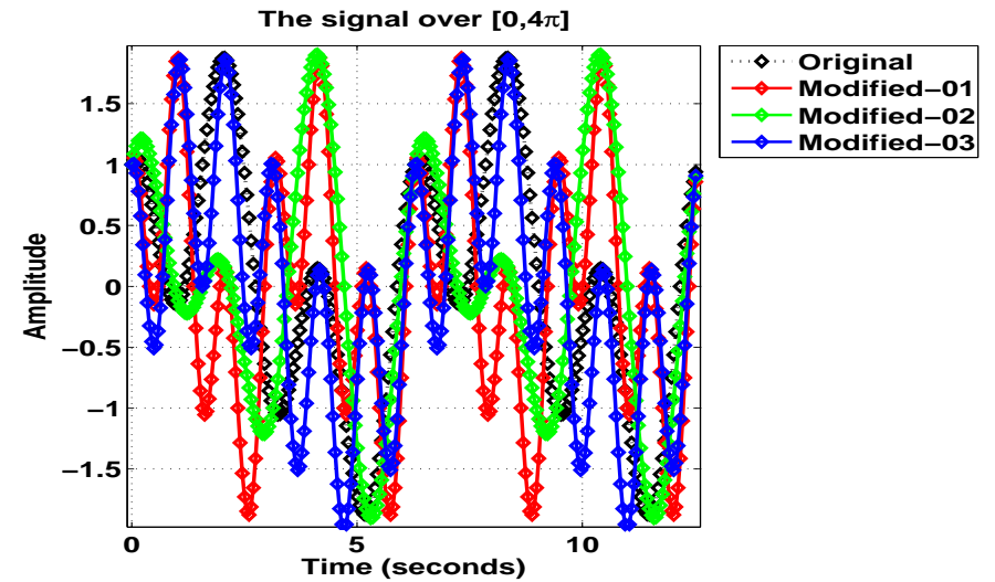
Figure: Comparison of f_0(t) , f_1(t) , f_2(t) , and f_3(t) .
