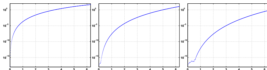
E_5(x)
