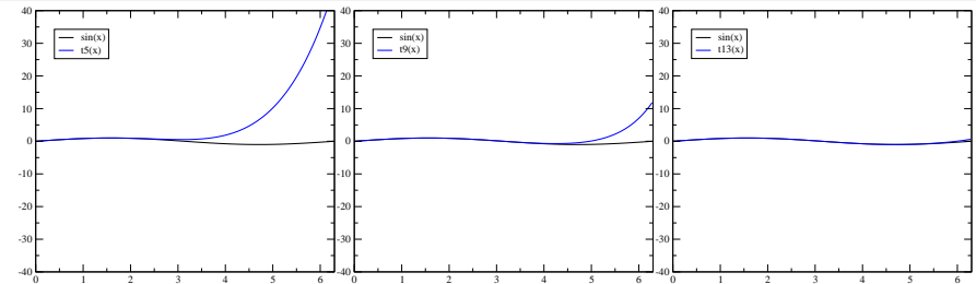
P_5(x)
