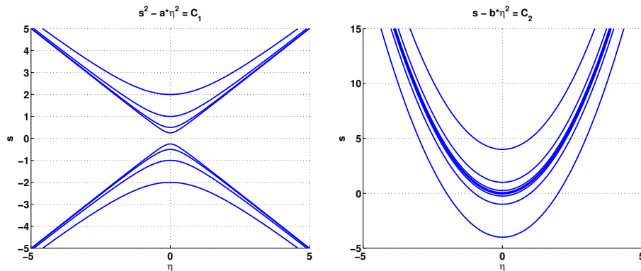
Figure: [LEFT] The hyperbolas s^2 - a^2 \eta^2 = C_h in the (\eta, s) -plane; and [RIGHT] the parabolas s - b \eta^2 = C_p in the (\eta, s) -plane.
