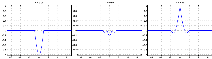
Figure: Snapshots at T = 0 , T = 0.5 , and T = 1.0 . See also the movie wave03.mpg
