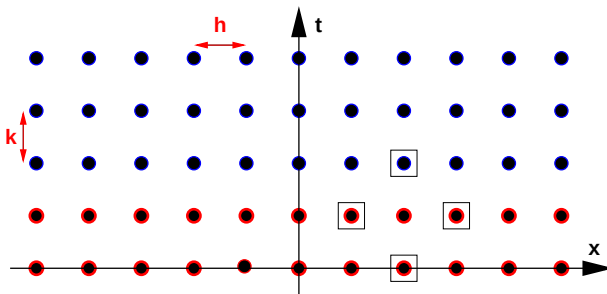
Figure: Once the first two levels v_m^0 , and v_m^1 are defined using the initial conditions v_m^0 = u_0(x_m) and some other clever initialization scheme for v_m^1 , on the red grid-points, a two-step scheme, such as the Leapfrog scheme
