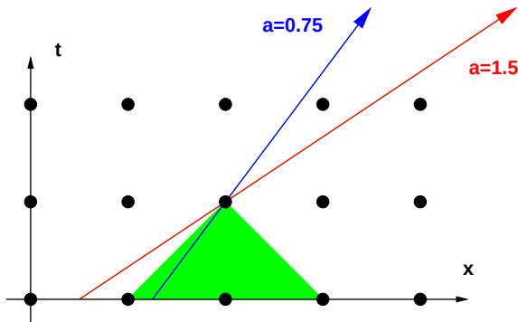
Figure: Illustration of the CFL condition, with \lambda = 1 held fixed. The green triangle shows the region of dependence, i.e. what region influences v_m^{n+1} (actually only the three points at the base of the triangle contribute). The blue arrow corresponds to a characteristic with speed a = 0.75 , which carries information inside the region of dependence; the red arrow, corresponding to a characteristic speed of a = 1.5 carries information from outside the region of dependence — this information cannot be captured by the scheme.
